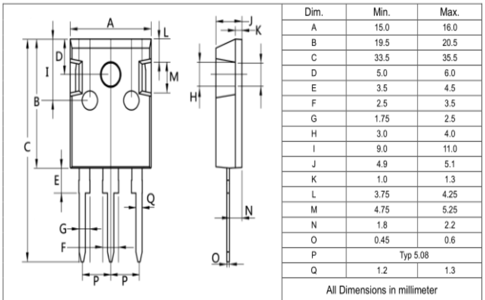
TO-247S
