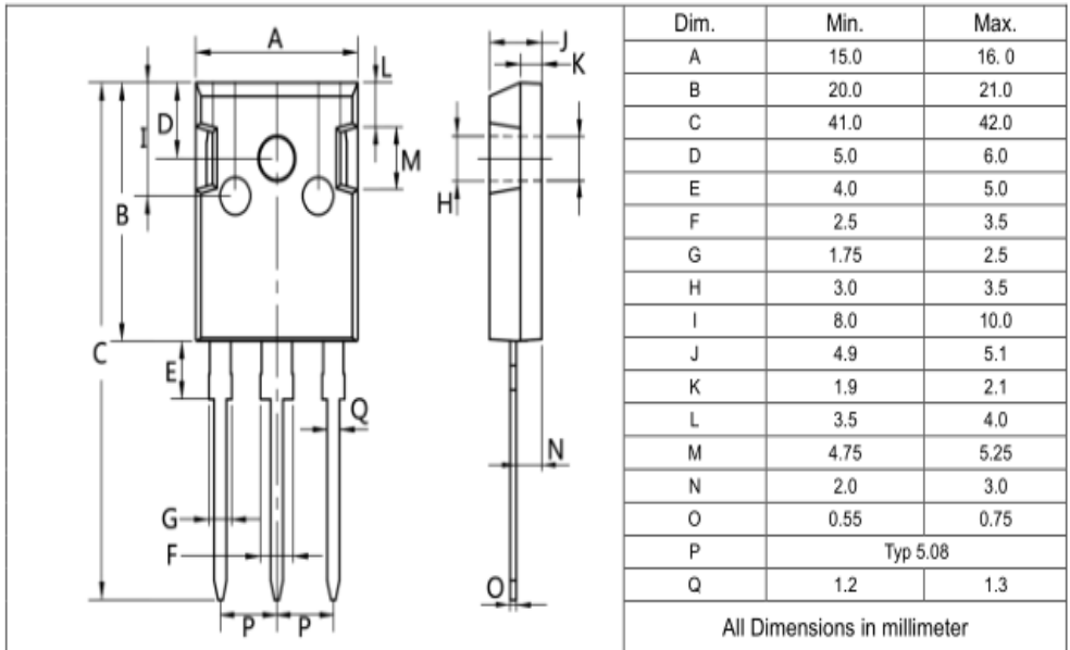
TO-247S
